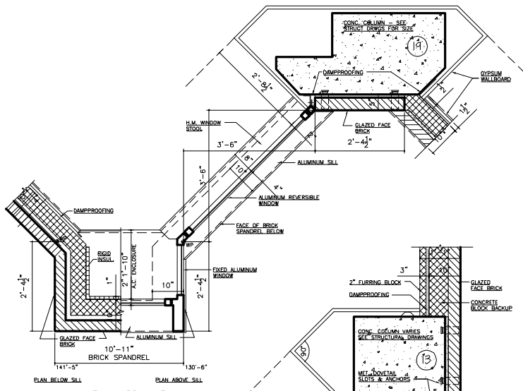
PLAN BELOW SILL BAY WINDOW UNIT AT 2ND FLOOR
