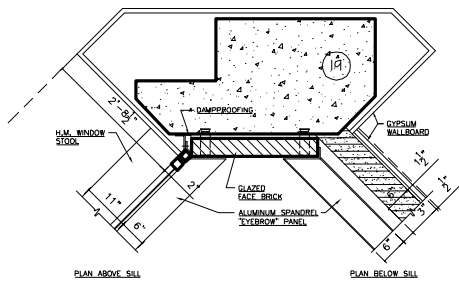
PLAN ABOVE SILL ENCLOSURE AT COLUMN 19 TYPICAL AT 3RD - 12TH FLOORS
