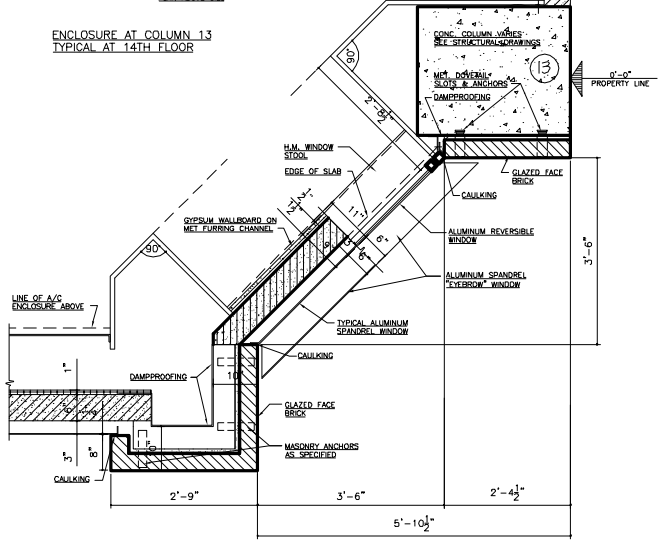
TYPICAL PIER ENCLOSURE AT 2ND FLOOR SPLAYED (45°) WINDOWS
