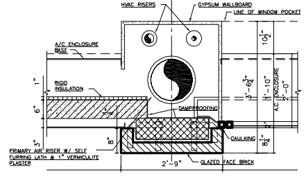
PLAN BELOW SILL TYPICAL HVAC ENCLOSURE AT WINDOWS
