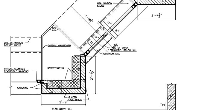
ENCLOSURE AT COLUMN 13 TYPICAL AT 14TH FLOOR
