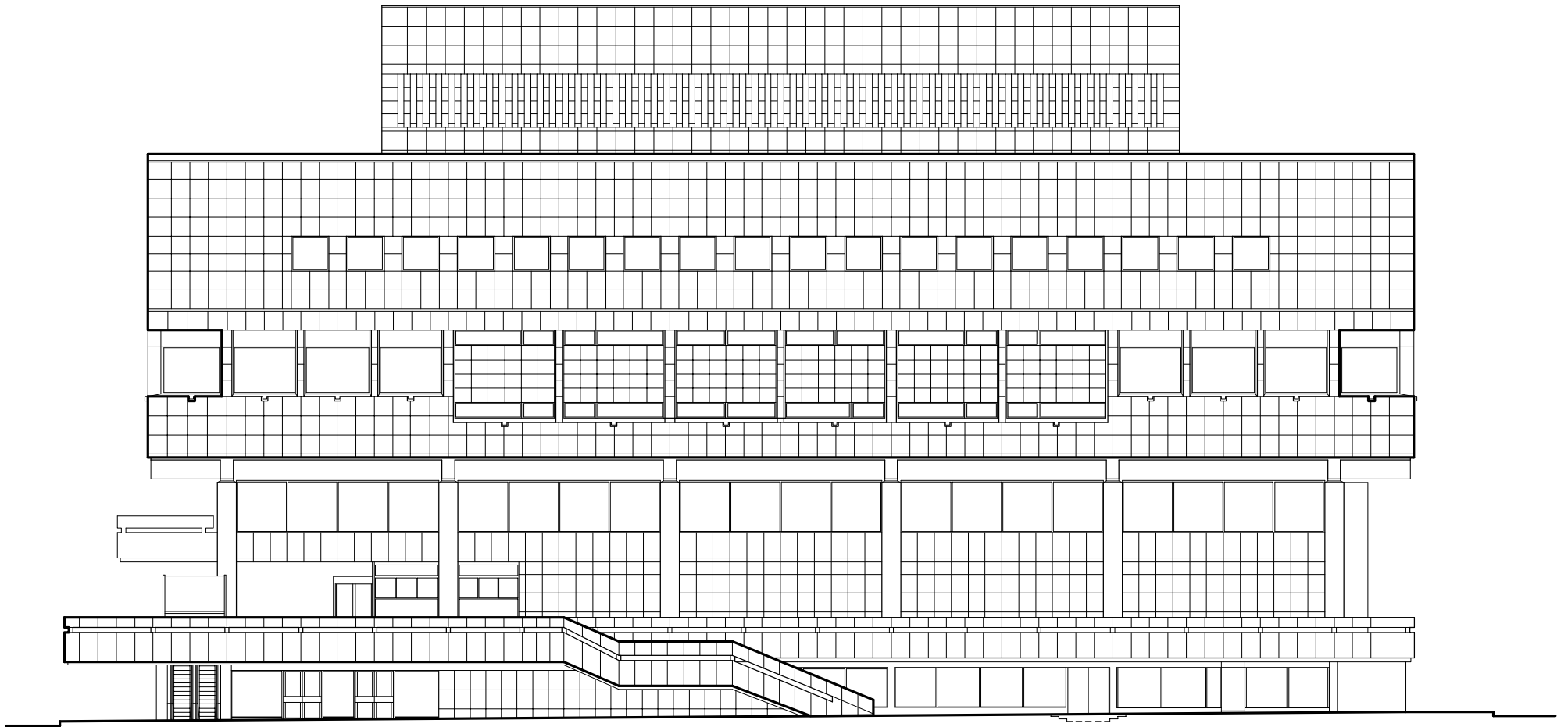
East Elevation Juilliard School & Alice Tully Hall New York, NY
